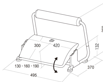
Figure 3.2 — 3185AT measurement drawing (dimensions in mm)
