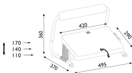
Figure 3.1 — 3184AT measurement drawing (dimensions in mm)
